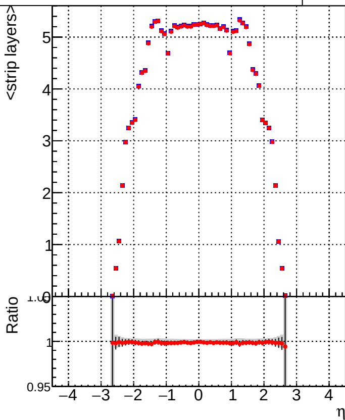
mean # STRIP Layers with measurement vs eta
