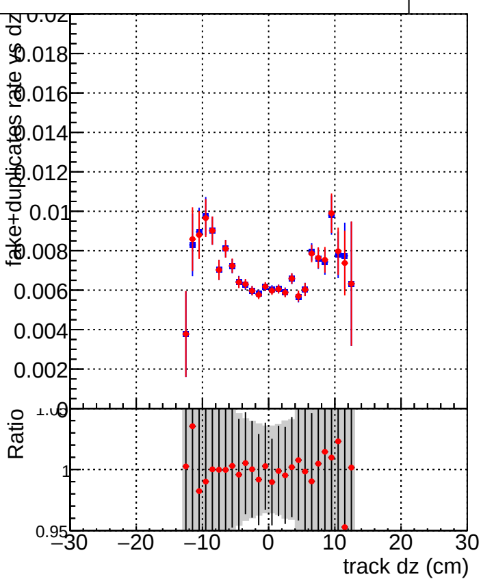
/home/data2/legianni/code-recovery/fitReview-forPR/test169+Fit/redo/CMSSW_16_0_X_2025-11-25-1100/s
