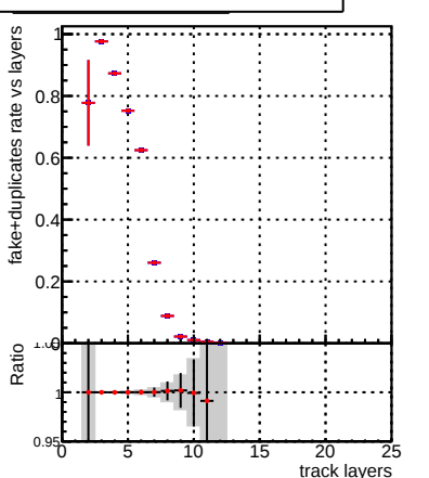
fake+duplicates rate vs layers
