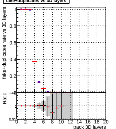
fake+duplicates rate vs 3D layers
