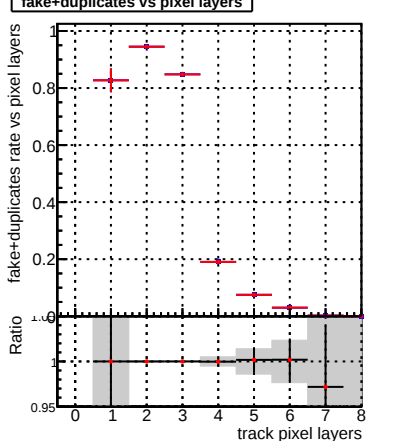
fake+duplicates rate vs pixel layers
