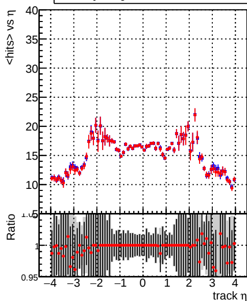
mean hit — DQM_SingleMuPt1_mkFit_Build — DQM_SingleMuPt1_mkFit_BuildNEW
