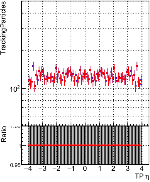
■ DQM_SingleMuPt10_mkFit_build ● DQM_SingleMuPt10_mkFit_BuildNEW
