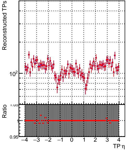
■ DQM_SingleMuPt10_mkFit_build ● DQM_SingleMuPt10_mkFit_BuildNEW
