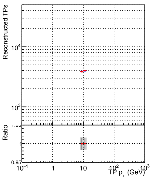
■ DQM_SingleMuPt10_mkFit_build ● DQM_SingleMuPt10_mkFit_BuildNEW
