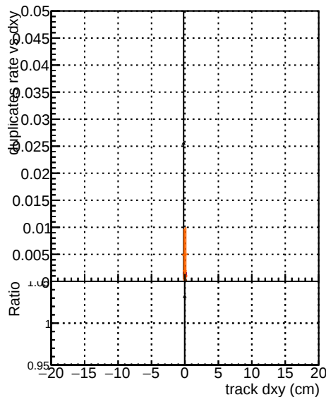
rescaleBoth
