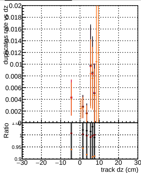
rescaleBoth
