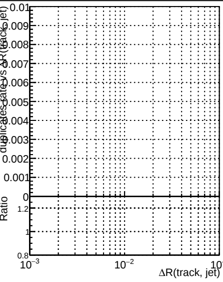
Fake rate vs \Delta R(\text{track}, \text{jet}) Duplicates Rate vs \Delta R(\text{track}, \text{jet}) Pileup rate vs \Delta R(\text{track}, \text{jet}) Fake rate vs PU Duplicates Rate vs PU Pileup rate vs PU
