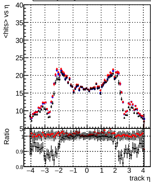
DQM_SingleMuPt1_mkFit_BuildNEW2 DQM_SingleMuPt1_mkFit_FitNEW2 DQM_SingleMuPt1_mkFit_NoFitNEW2 mean hits
