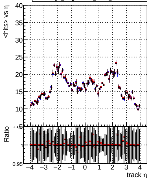
mean hits — DQM_SingleMuPt1_mkFit_BuildNEW2 — DQM_SingleMuPt1_mkFit_FitNEW2 — DQM_SingleMuPt1_mkFit_NoFitNEW2
