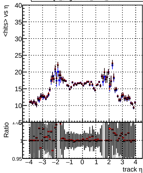
mean hits vs \eta DQM_SingleMuPt1_mkFit_BuildNEW2 DQM_SingleMuPt1_mkFit_FitNEW2 DQM_SingleMuPt1_mkFit_NoFitNEW2
