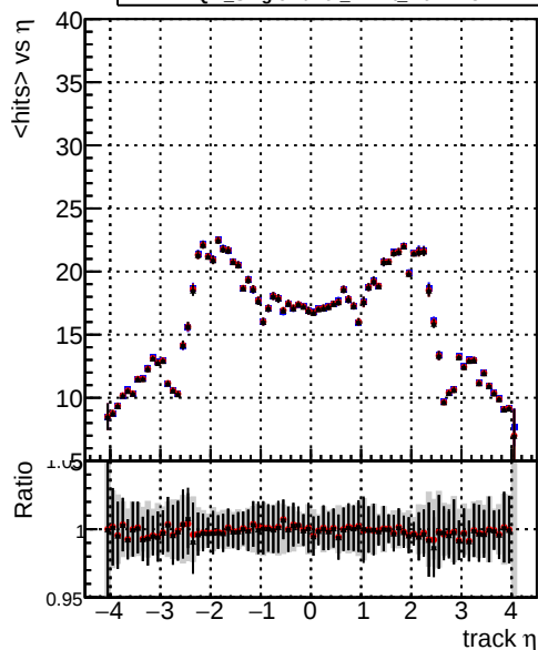
mean hit — DQM_SingleMuPt1_mkFit_BuildNEW2 — DQM_SingleMuPt1_mkFit_FitNEW2 — DQM_SingleMuPt1_mkFit_FitNEW3
