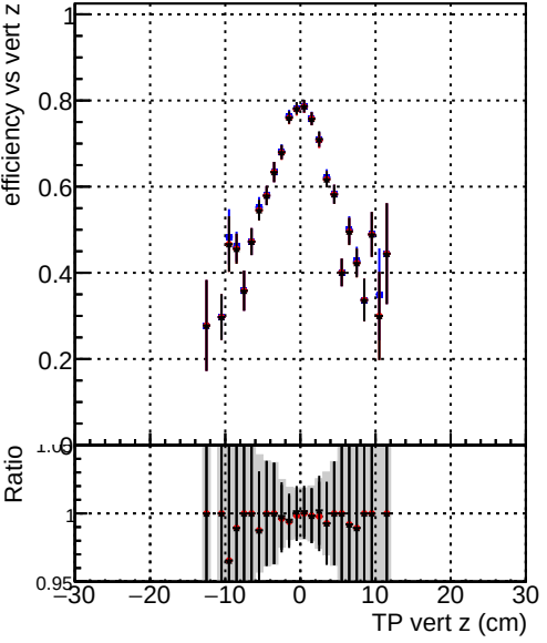
Efficiency vs. TP vert z (cm) Legend: DQM_SingleMuPt1_mkFit_BuildNEW2 (blue line with circles) DQM_SingleMuPt1_mkFit_FitNEW2 (red line with circles) DQM_SingleMuPt1_mkFit_FitNEW3 (black line with circles)
