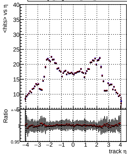
mean hits — DQM_SingleMuPt1_mkFit_BuildNEW2 — DQM_SingleMuPt1_mkFit_FitNEW2 — DQM_SingleMuPt1_mkFit_FitNEW3
