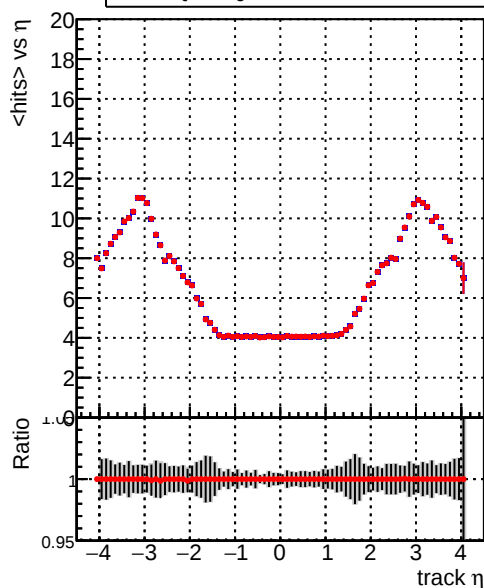
mean hits — DQM_SingleMuPt1_mkFit_BuildNEW2 — DQM_SingleMuPt1_mkFit_FitNEW2
