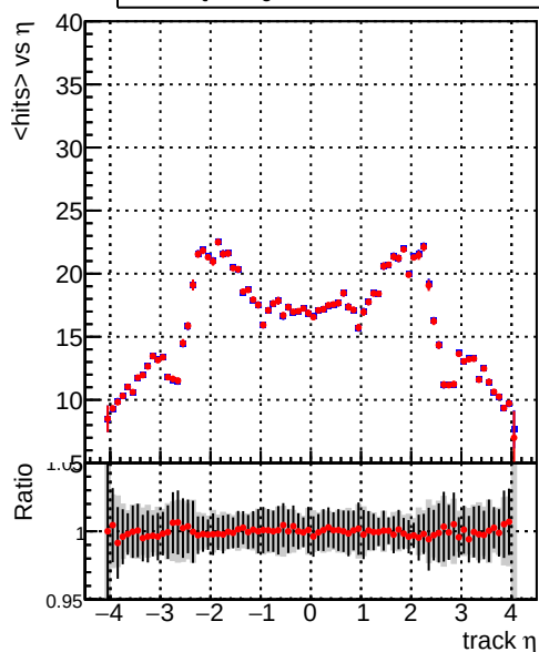
mean hit — DQM_SingleMuPt1_mkFit_BuildNEW2 — DQM_SingleMuPt1_mkFit_FitNEW2
