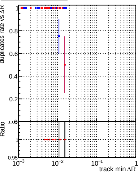
Legend: DQM_SingleMuPt1_mkFit_BuildNEW2 DQM_SingleMuPt1_mkFit_FitNEW2
