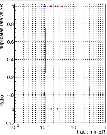
DQM_SingleMuPt1_mkFit_BuildNEW DQM_SingleMuPt1_mkFit_FitNEW
