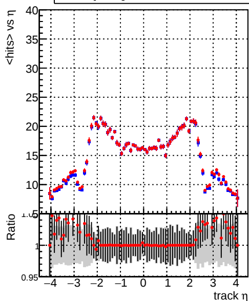
mean hits vs \eta — DQM_SingleMuPt1_mkFit_Build — DQM_SingleMuPt1_mkFit_BuildNEW2
