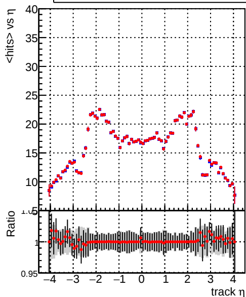
mean hits — DQM_SingleMuPt1_mkFit_build — DQM_SingleMuPt1_mkFit_BuildNEW2
