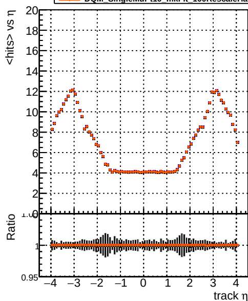
mean hits vs \eta Legend: DOM_SingleMuPt10_mkFit_build (Blue line with circles) DOM_SingleMuPt10_mkFit_Fit (Red line with circles) DOM_SingleMuPt10_mkFit_100RescaleBack (Black line with circles) DOM_SingleMuPt10_mkFit_100RescaleHalf (Orange line with circles)
