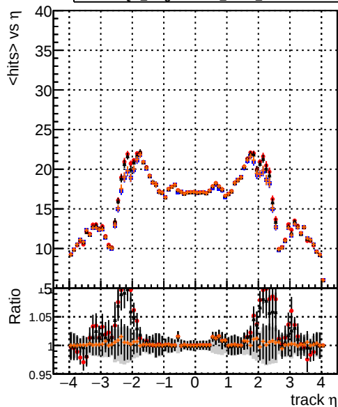
DOM_SingleMuPt10_mkFit_build DOM_SingleMuPt10_mkFit_Fit DOM_SingleMuPt10_mkFit_100RescaleBoth DOM_SingleMuPt10_mkFit_NoFit mean hits
