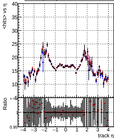
mean hit — DQM_SingleMuPt10_mkFit_BuildNEW — DQM_SingleMuPt10_mkFit_FitNEW — DQM_SingleMuPt10_mkFit_NoFitNEW
