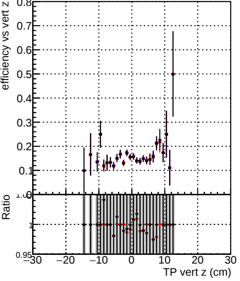
Efficiency vs TP vert z Legend: DQM_SingleMuPt10_mkFit_BuildNEW2 DQM_SingleMuPt10_mkFit_FitNEW2 DQM_SingleMuPt10_mkFit_FitNEW3
