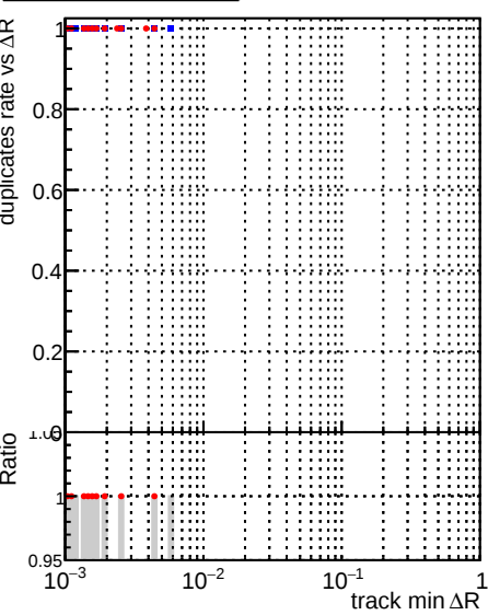
DQM_SingleMuPt10_mkFit_BuildNEW2 DQM_SingleMuPt10_mkFit_FitNEW2
