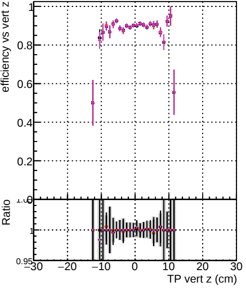
Efficiency vs. TP vert z (cm) Legend: DOM SingleMuPt10 mkFit build DOM SingleMuPt10 mkFit Mt DOM SingleMuPt10 mkFit NotFlexible DOM SingleMuPt10 mkFit simplifiedMF DOM SingleMuPt10 mkFit NoStripCPE
