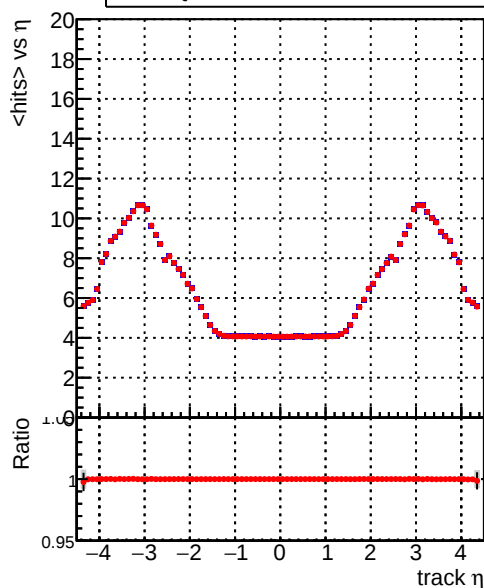
mean hits vs \eta Legend: DQM_TTPU_mkFit_BuildNEW4 (blue line), DQM_TTPU_mkFit_FitNEW4 (red line)
