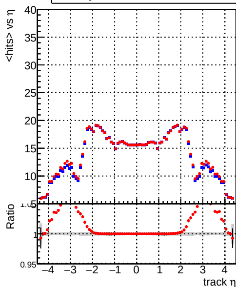
mean hits vs \eta Legend: DQM_TTPU_mkFit_Build (blue line), DQM_TTPU_mkFit_BuildNEW3 (red line)
