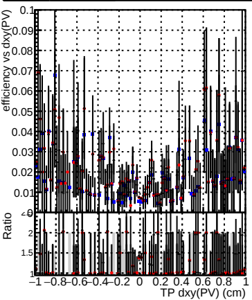
Efficiency vs Dxy(PV) Legend: DQM_V0001_R000000001_Global_CKF_RECO DQM_V0001_R000000001_Global_mkFit1_RECO DQM_V0001_R000000001_Global_mkFit2_RECO
