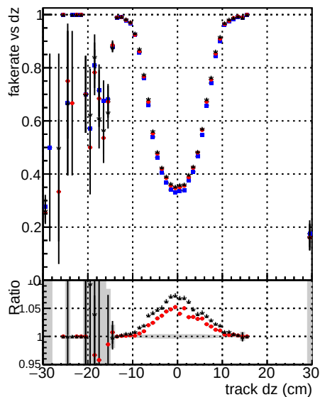
Fake rate vs d DOM V0001 R0000000001 Global CKF RECO Global MKFI2 RECO
