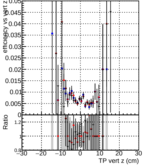
Efficiency vs vert z Global_CKF_RECO Global_mkFit1_RECO Global_mkFit2_RECO
