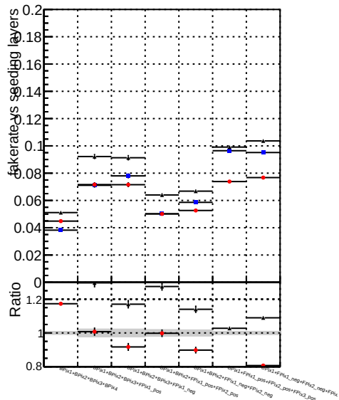
Fake rate vs. DOM V0001 R0000000001 Global CKF RECO DOM V0001 R0000000001 Global mktF12 RECO
