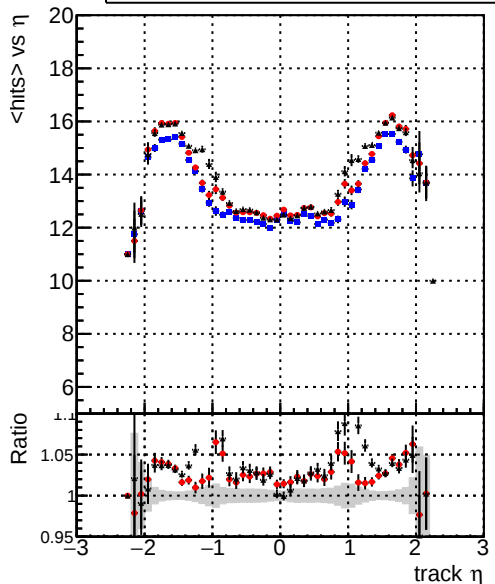
DQM_V0001_R000000001_Global_CKF_RECO DQM_V0001_R000000001_Global_mkFit1_RECO DQM_V0001_R000000001_Global_mkFit2_RECO mean hits
