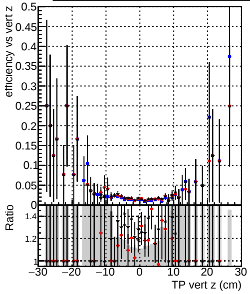
Efficiency vs. sim PV z Global_CKF_RECO Global_mkFit1_RECO Global_mkFit2_RECO
