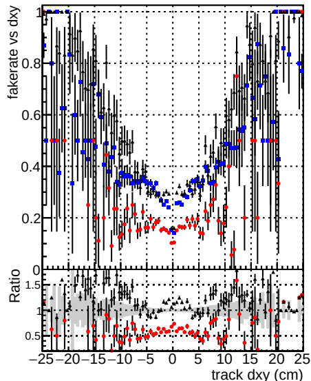
DOM V0001 DOM V0001 RECO Global CKF RECO Fake rate vs d Blue diamonds Red diamonds Black crosses Blue diamonds Red diamonds Duplicates Rate vs Dxy Blue diamonds Red diamonds Black crosses Blue diamonds Red diamonds Pileup rate vs dxy Blue diamonds Red diamonds Black crosses Blue diamonds Red diamonds Fake rate vs dz Blue diamonds Red diamonds Black crosses Blue diamonds Red diamonds Duplicates Rate vs Dxy Blue diamonds Red diamonds Black crosses Blue diamonds Red diamonds Pileup rate vs dxy Blue diamonds Red diamonds Black crosses Blue diamonds Red diamonds
