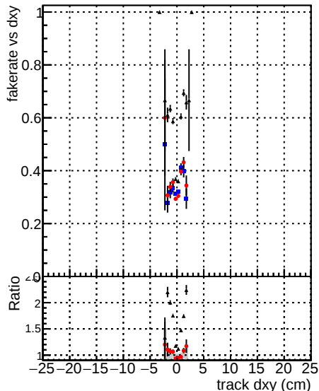
DOM V0001 DOM V0001 RECO Global CKF RECO Global mkFit RECO Fake rate vs d
