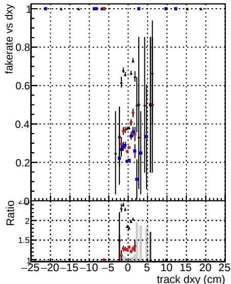
DOM V0001 DOM V0001 RECO Global RECO Fake rate vs d Blue circles Red circles Black circles Duplicates Rate vs Dxy Blue circles Red circles Black circles Pileup rate vs dxy Blue circles Red circles Black circles
