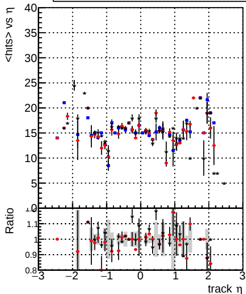
DQM_V0001_R000000001_Global_CKF_RECO DQM_V0001_R000000001_Global_mkFit1_RECO DQM_V0001_R000000001_Global_mkFit2_RECO
