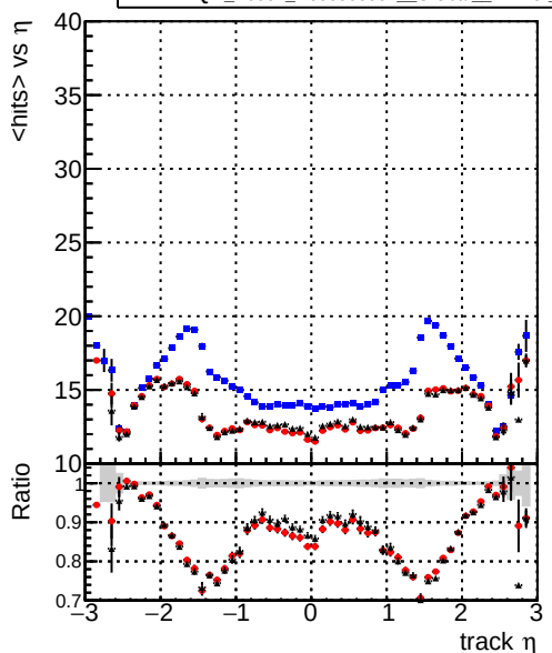
— DQM_V0001_R000000001_Global_CKF_RECO — DQM_V0001_R000000001_Global_mkFit1_RECO — DQM_V0001_R000000001_Global_mkFit2_RECO
