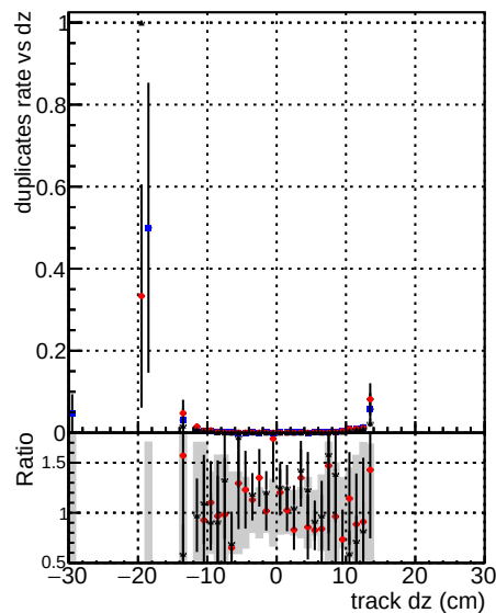
DOM V0001 R0000000001 Global CKF RECO DOM V0001 R0000000001 Global mkFit2 RECO
