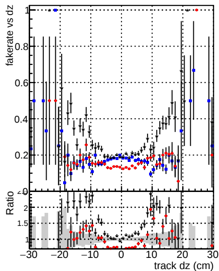
Fake rate vs dz DOM V0001 R0000000001 Global CKF RECO DOM V0001 R0000000001 Global mkt12 RECO
