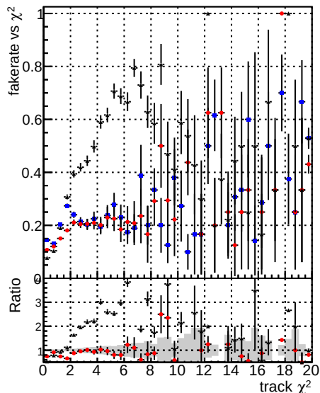
Fake rate vs. DOM V0001 R0000000001 Global CKE RECO Global DOM V0001 R0000000001 Global CKE RECO
