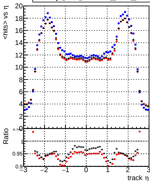
mean hits — DQM_V0001_R000000001_Global_CKF_RECO — DQM_V0001_R000000001_Global_mkFit1_RECO — DQM_V0001_R000000001_Global_mkFit2_RECO
