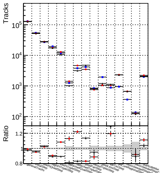
Number of tracks vs collection DQM_V0001_R000000001_Global_CKF_RECO DQM_V0001_R000000001_Global_mkFit1_RECO DQM_V0001_R000000001_Global_mkFit2_RECO
