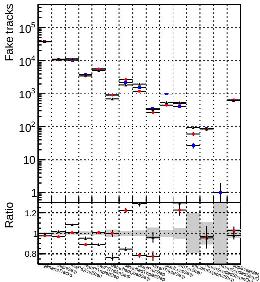
Number of tracks vs collection DQM_V0001_R000000001_Global_CKF_RECO DQM_V0001_R000000001_Global_mkFit1_RECO DQM_V0001_R000000001_Global_mkFit2_RECO
