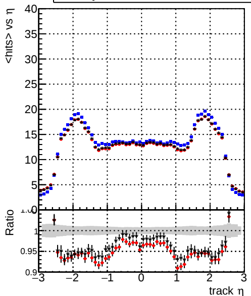
mean hit — DQM_V0001_R000000001_Global_CKF_RECO — DQM_V0001_R000000001_Global_mkFit1_RECO — DQM_V0001_R000000001_Global_mkFit2_RECO
