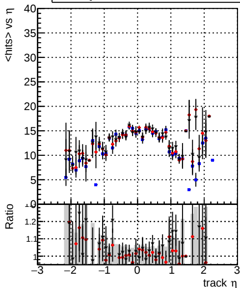
mean hit — DQM_V0001_R000000001_Global_CKF_RECO — DQM_V0001_R000000001_Global_mkFit1_RECO — DQM_V0001_R000000001_Global_mkFit2_RECO
