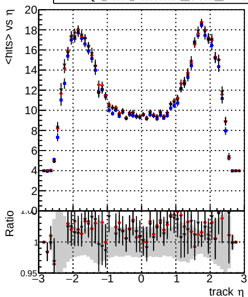
mean hits vs \eta Legend: DQM_V0001_R000000001_Global_CKF_RECO (blue line), DQM_V0001_R000000001_Global_mkFit1_RECO (red line), DQM_V0001_R000000001_Global_mkFit2_RECO (black line)
