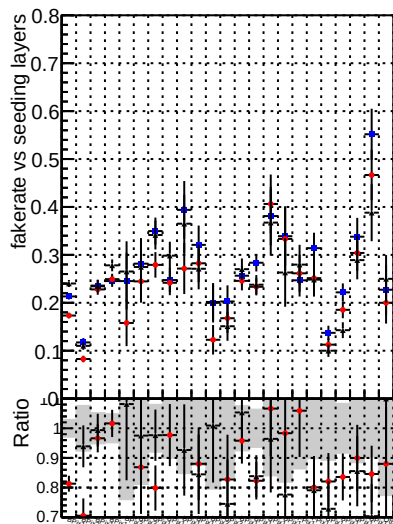
Fake rate vs. Legend DOM V0001 DOM V0001 R0000000001 Global CKF RECO RECO Line Blue Red Black Blue Red Point Blue Red Black Blue Red Ratio Blue Red Black Blue Red
