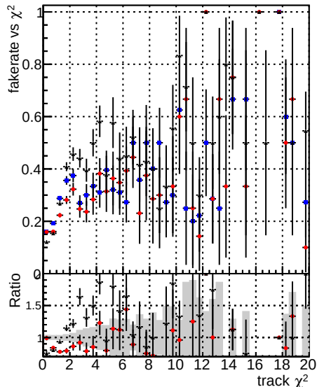
Fake rate vs. Legend DOM V0001 DOM V0001 R0000000001 Global CKF RECO RECO Line Blue Red Black Blue Red Point Blue Red Black Blue Red Ratio Blue Red Black Blue Red
