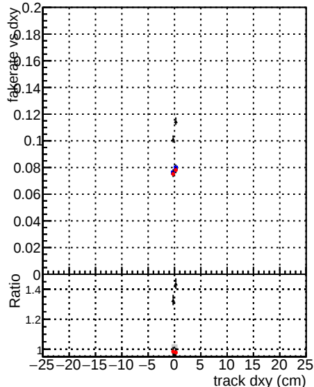
DOM V0001 DOM V0001 Global CKF RECO Fake rate vs d Blue line with dots Red line with dots Black line with dots Blue line with dots Red line with dots Duplicates Rate vs dxy Blue line with dots Red line with dots Black line with dots Blue line with dots Red line with dots Pileup rate vs dxy Blue line with dots Red line with dots Black line with dots Blue line with dots Red line with dots
