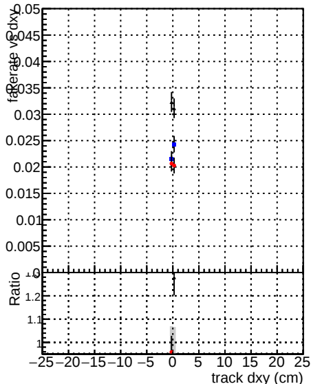
DOM V0001 DOM V0001 RECO Global CKF RECO Global mkFit2 RECO Fake rate vs d Blue line with dots Red line with dots Black line with dots Blue line with dots Red line with dots Black line with dots
