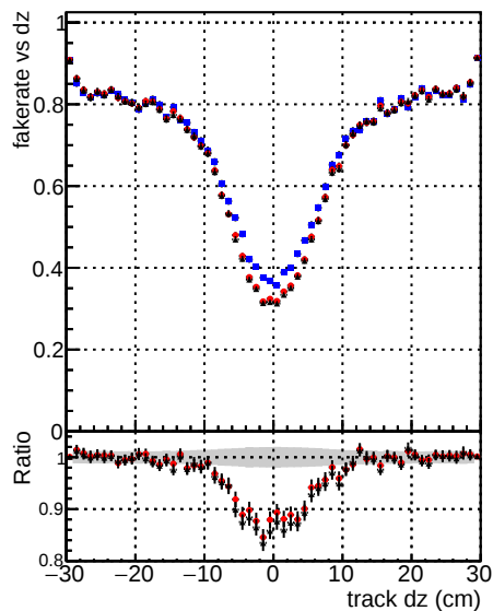
DOM V0001 DOM V0001 RECO Global RECO Fake rate vs d Blue squares Red circles Black line Duplicates Rate vs Dxy Blue squares Red circles Black line Pileup rate vs dxy Blue squares Red circles Black line
